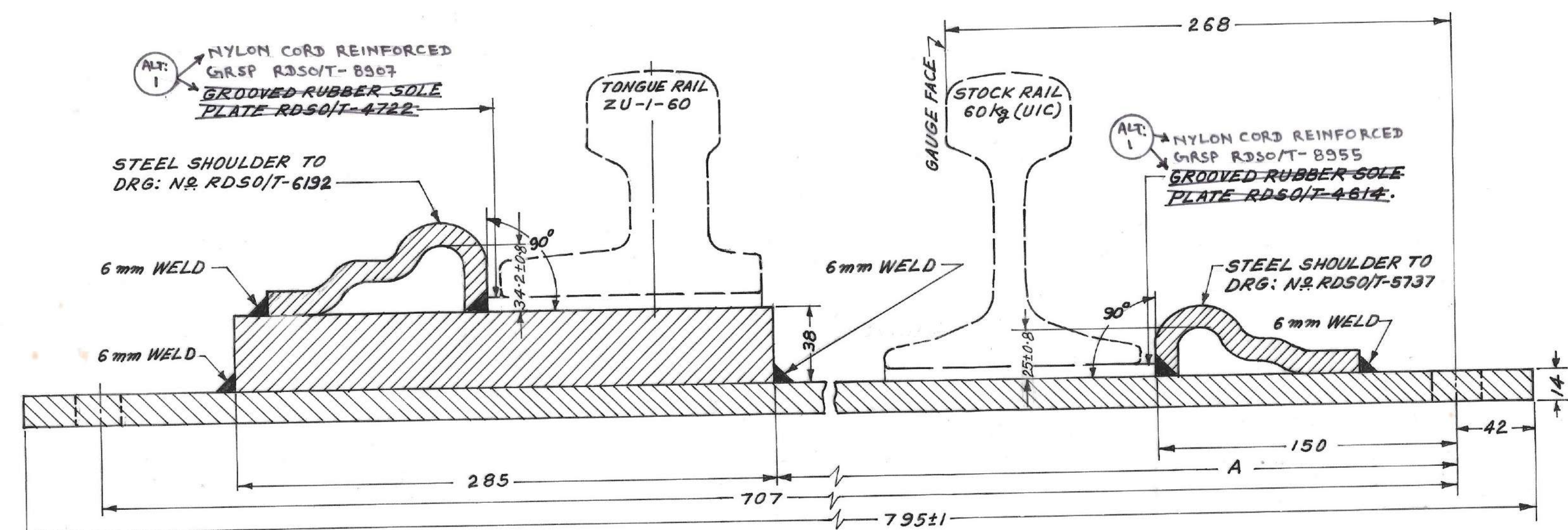
SECTIONAL ELEVATION ON A.B.
